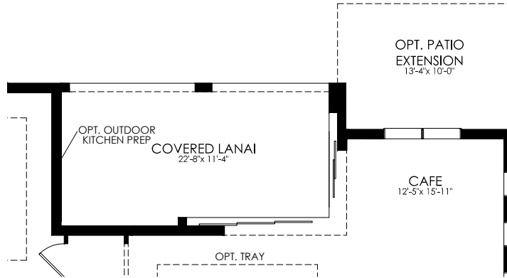
Zero Corner SGD at Gathering Room
