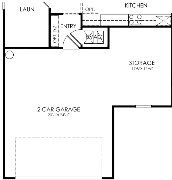
4' Garage Extension
